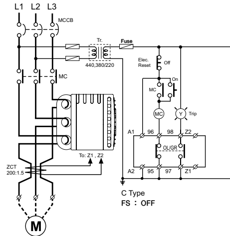
Three phase motor (C type, common output)
